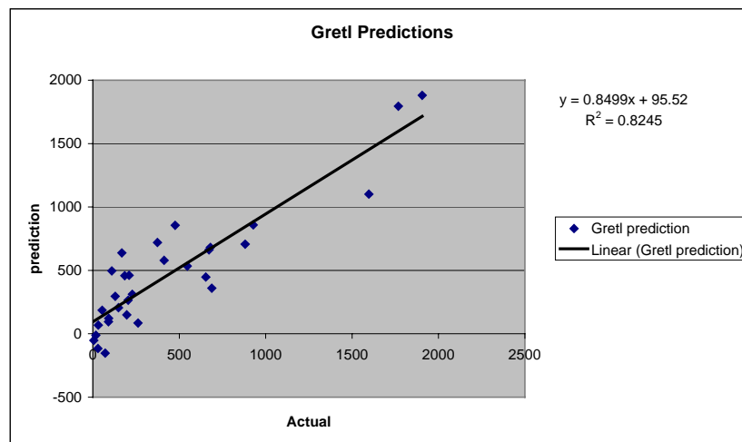
Figure 10 Regression model defect counts against actuals
