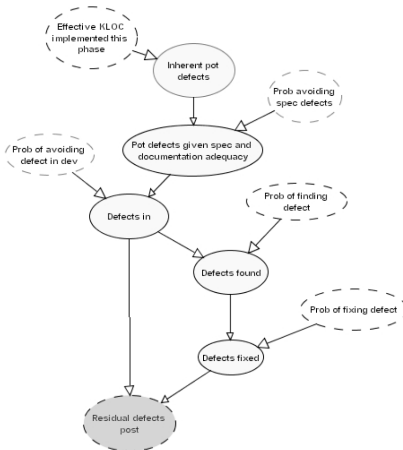
Figure 1 BN for Defect Prediction
