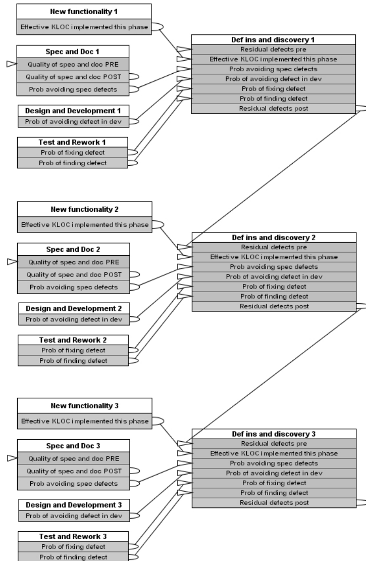
Figure 6 An Incremental Development Lifecycle
