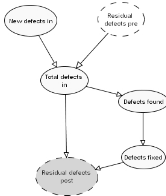
Figure 2 A Dynamic BN Modelling a Software Lifecycle
