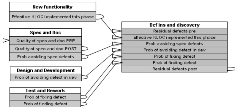
Figure 3 Objects in the Phase BN
