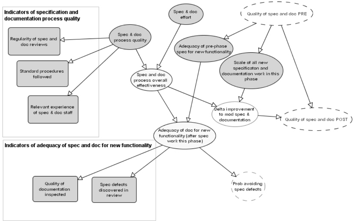
Figure 4 Specification and Documentation Class
