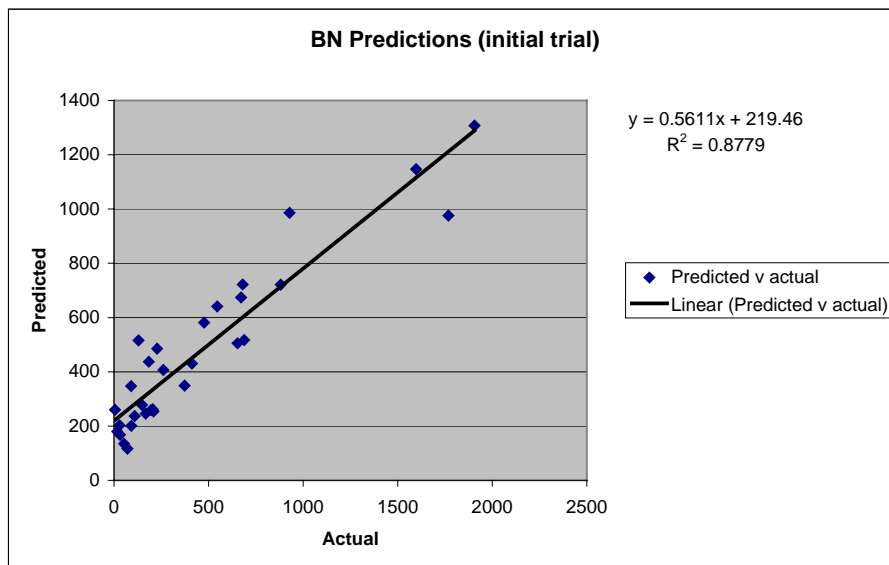
Figure 9 Predicted verses actual defects (initial trial)
