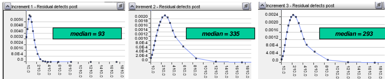
Figure 7 Defects Predicted at Each Increment of the Incremental Lifecycle
