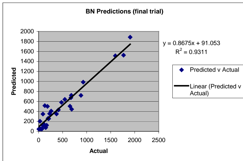
Figure 11 Two phase prediction result
