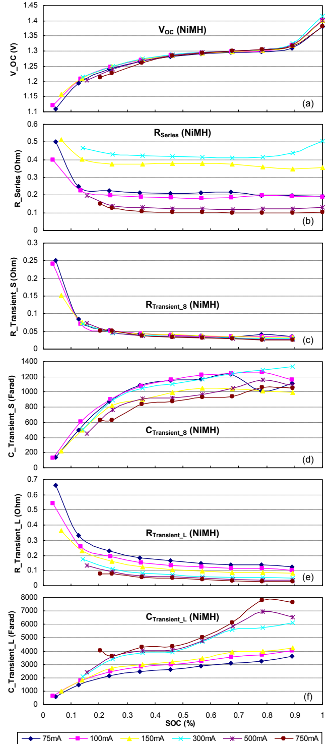
Fig. 10. Extracted parameters of the NiMH battery at room temperature.
